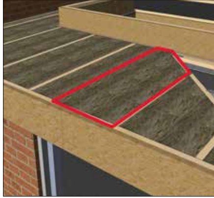
Lay a bead of glue under the first board which is positioned next to the hip and kerb. The hip mitre of the board should line up with the centre of the hip firring. Fitter's tip: Lay the boards out around the hip before gluing to trial where they need to be placed.
