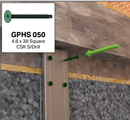
Detail Specific to hup! jobs. Fix the internal clips into the wall panels and beams using 4x GPHS050 screws. Fix 2 of the screws into the beam and the remaining 2 into the wall panel as shown. Do this on each box beam.
