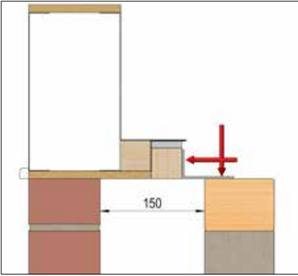
For 150mm cavities, a box beam holding down bracket will be provided to be fit at 600mm centres, 2 fixings into beam using NRDS070 and 2 fixings into timber wall plate through the pre-drilled holes (NOT SUPPLIED).
