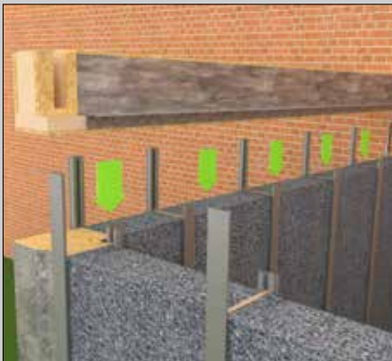
Detail Specific to hup! jobs. Lower the box beam between the internal and external clips until it sits on the wall panels. Prop if needed.
