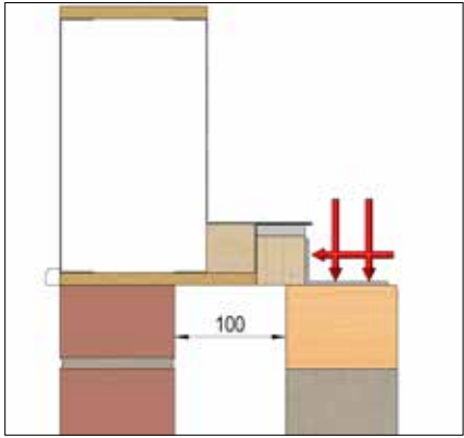
For 100mm cavities, a box beam holding down bracket will be provided to be fit at 600mm centres, 2 fixings into beam using NRDS070 and 4 fixings into timber wall plate through the pre-drilled holes (NOT SUPPLIED).
