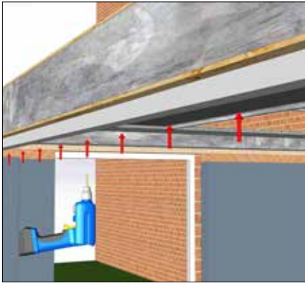
Any frames should be fixed into the underside of the beam through the frame. Fixings should be within 150mm of each corner and at max. 450mm centres using suitable fixings (NOT SUPPLIED).
