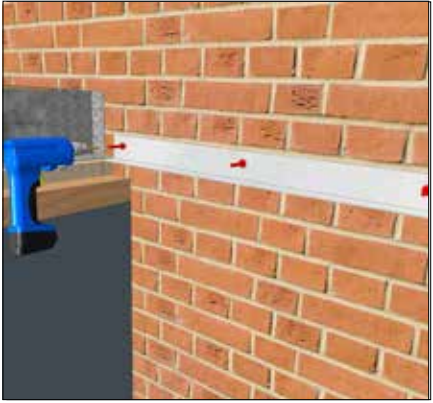
Line up the wall plate with the beam shelf so it sits flush. Fix the longest side of the wall plate to the host wall, 200mm from ends and at maximum 450mm centres. Avoid mortar joints and use appropriate fixings (NOT SUPPLIED).
