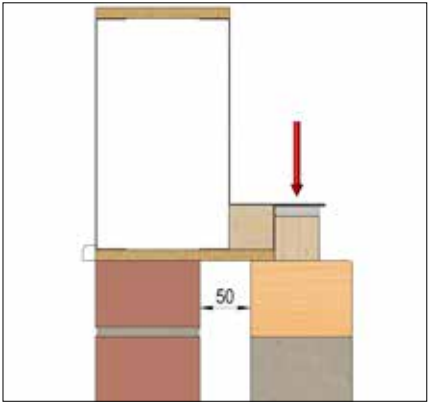
For 50mm cavities, the gap between the timber and the shelf should be packed out and the beam should be fixed down into the timber wall plate through the shelf at 300mm centres with suitable fixings (NOT SUPPLIED).
